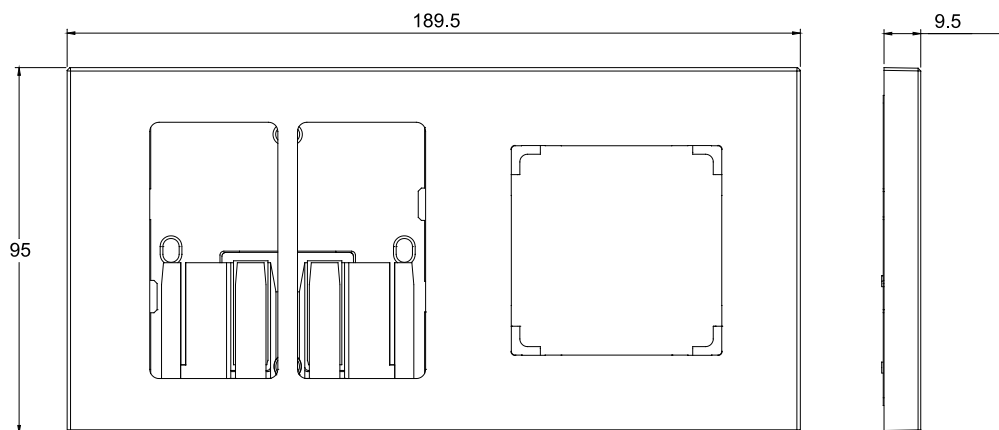
Frame Dimensions
